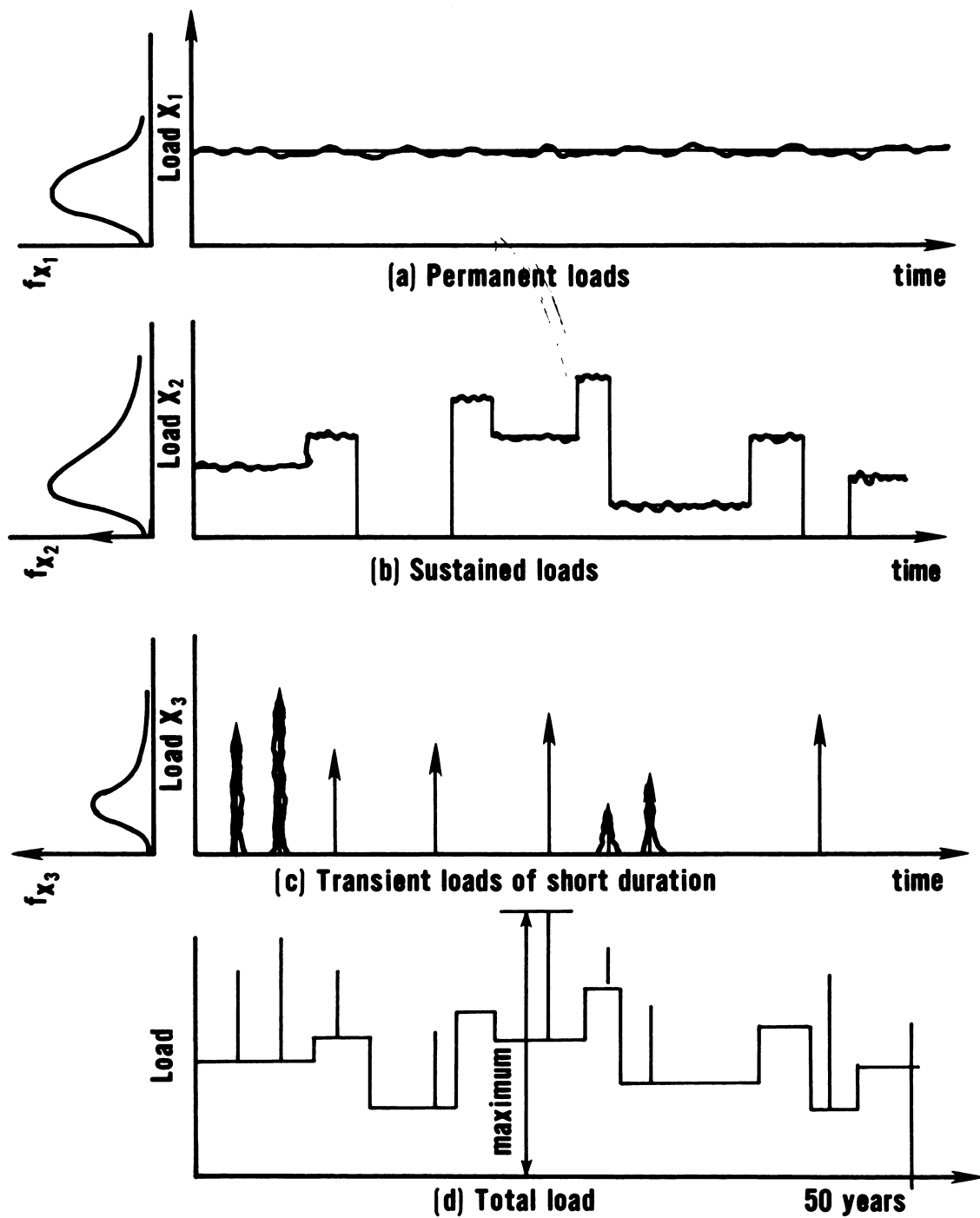
Figure 2.5 - Typical Load Process Models
