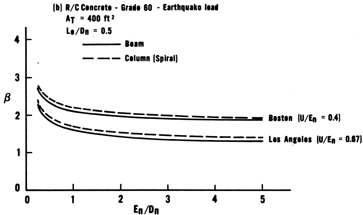
Figure 4.6 - Reliability Index for Steel and Reinforced Concrete Beams - Gravity Plus Earthquake Load ( 100 \text{ ft}^2 = 9.3 \text{ m}^2 )
