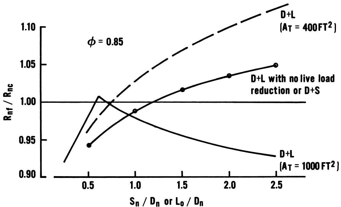
Figure 5.11b HOT-ROLLED STEEL BEAMS - GRAVITY LOADS
