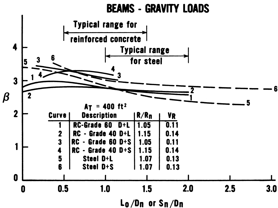
Figure 4.1 - Reliability Index for Steel and Reinforced Concrete Beams Conforming to Current Criteria - Gravity Loads ( 100 \text{ ft}^2 = 9.3 \text{ m}^2 )
