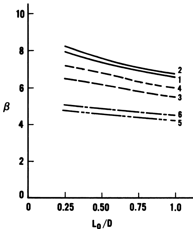
Figure 4.2 - Reliability Index for Nonreinforced Brick and Concrete Masonry Walls Conforming to Current Criteria ( 100 \text{ ft}^2 = 9.3 \text{ m}^2 )
